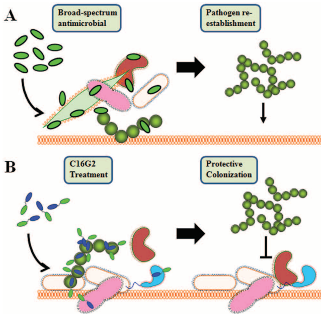
Figure 1. Illustration of targeted antimicrobial treatment for long-term protection. (A) Broad-spectrum antimicrobial therapy results in killing of pathogenic and normal flora bacteria. The mucosal surface can be re-colonized by pathogens. (B) Targeted STAMP (C16G2) treatment results in selective pathogen removal and protective colonization associated with the remaining and established normal flora.
