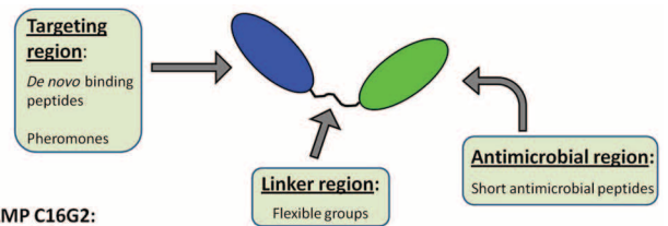
Figure 2. Illustration of the basic structure for the specifically targeted antimicrobial peptides (STAMPs). Adapted from Eckert (2011).
