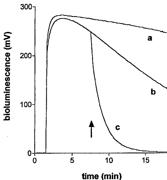
Figure 1. Luciferin-luciferase method for measuring ATP in saliva: bioluminescence curve (expressed as mV) related to the time (a) in the presence of 0.1 \text{ mM} vanadate, (b) in the absence of vanadate and (c) in the absence of vanadate with addition (indicated by an arrow) of 0.1 \text{ U} ATPase. The graph is representative of six independent experiments.
