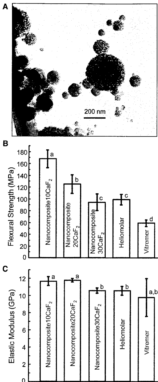
Figure 1. CaF 2 nanoparticles and composite mechanical properties before immersion. (A) TEM micrograph of the new CaF 2 nanopowder, with median particle size of 56 nm. (B) Flexural strength, and (C) elastic modulus, of nanocomposite, with dry specimens before immersion. Each value is the mean of 6 measurements, with the error bar showing 1 standard deviation (mean ± SD; n = 6). In each plot, bars with dissimilar letters indicate values that are significantly different from each other (p < 0.05).
