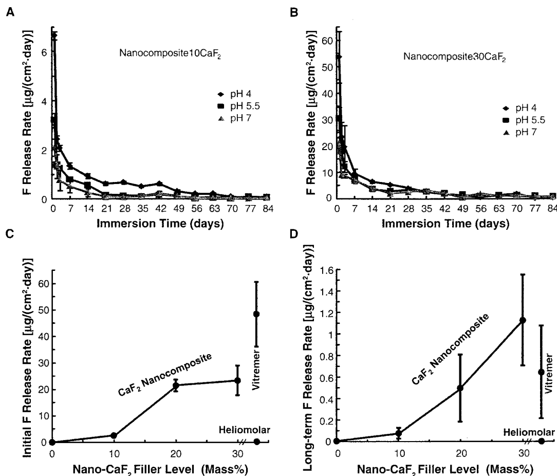
Figure 4. Fluoride release rate, which is the F release per specimen surface area per day (mean \pm SD; n = 3). Each error bar shows 1 standard deviation. (A) Nanocomposite10CaF 2 and (B) Nanocomposite30CaF 2 , (C) Initial F-release rates. Vitremer had the highest initial release [ 48.4 \pm 12.3 \mu\text{g}/(\text{cm}^2\cdot\text{day}) ], followed by 23.4 \pm 5.6 for Nanocomposite30CaF 2 , 21.5 \pm 2.2 for Nanocomposite20CaF 2 , 2.4 \pm 0.2 for Nanocomposite10CaF 2 , and 0.17 \pm 0.04 for Heliomolar ( p < 0.05 ). (D) Long-term F-release rates were 1.13 \pm 0.42 for Nanocomposite30CaF 2 , 0.65 \pm 0.43 for Vitremer, and 0.50 \pm 0.31 for Nanocomposite20CaF 2 ( p > 0.1 ). They were higher than 0.10 \pm 0.05 of Nanocomposite10CaF 2 and 0.006 \pm 0.003 of Heliomolar ( p < 0.05 ).
