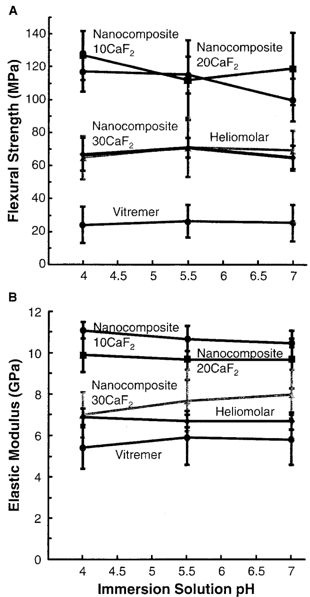
Figure 2. Mechanical properties after immersion. (A) Flexural strength, and (B) elastic modulus, of specimens immersed for 84 days in solutions of pH 4, pH 5.5, and pH 7. Each value is mean ± SD; n = 6. Each error bar shows 1 standard deviation. The nanocomposite with 10% nano-CaF 2 + 55% glass (Nanocomposite10CaF 2 ) and the nanocomposite with 20% CaF 2 + 45% glass (Nanocomposite20CaF 2 ) had the highest strengths. Heliomolar and the nanocomposite with 30% CaF 2 + 35% glass (Nanocomposite30CaF 2 ) had similar strengths, followed by that of Vitremer.
